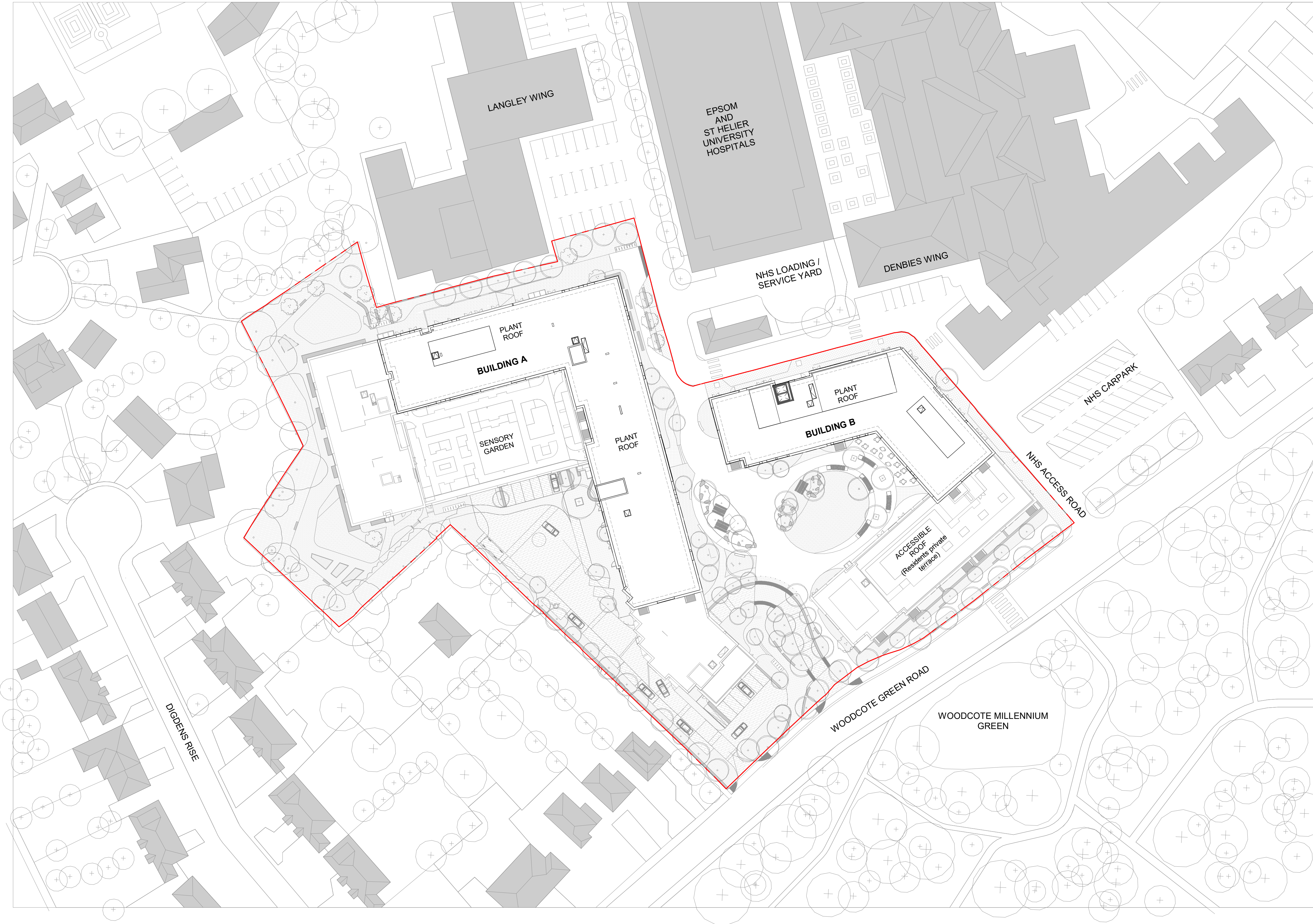
1 ROOF LEVEL MASTERPLAN 1 : 500
