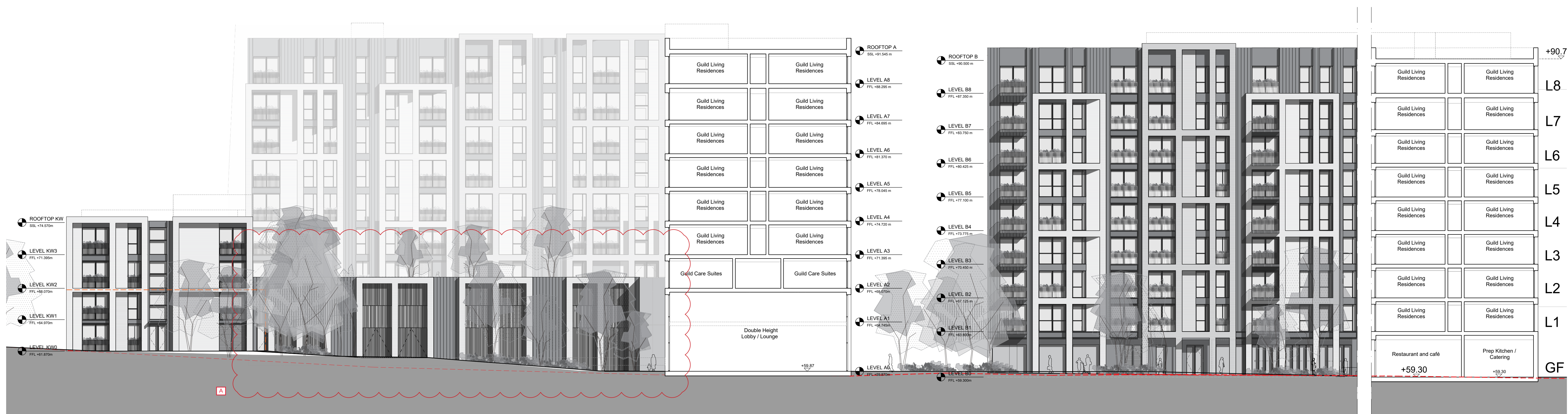
BUILDING SECTION AA'
